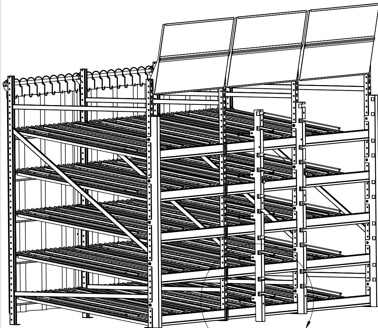
DETAIL C SCALE 1 : 10
