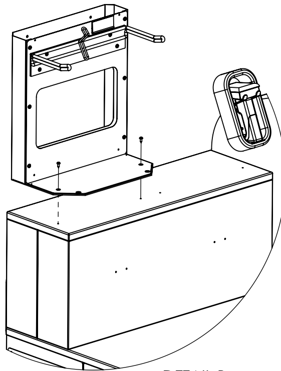
DETAIL B
